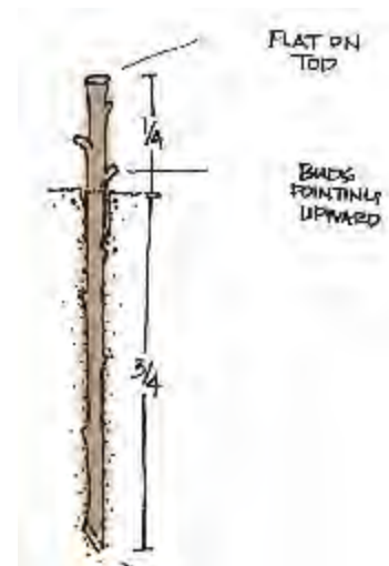
Figure 5: Livestake installation diagram
