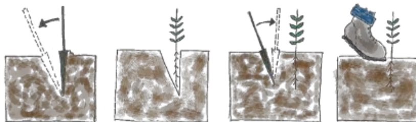
Figure 6: Emergent bareroot plug installation diagram
